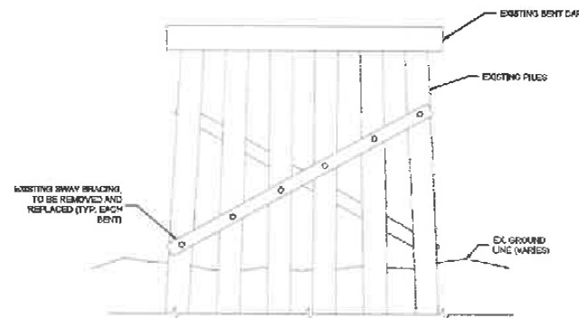
TYPICAL BENT ELEVATION 3 1"=20'-0" S1.0
