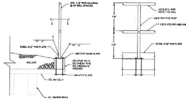
HANDRAIL DETAIL 2 1" = 1'-0"
