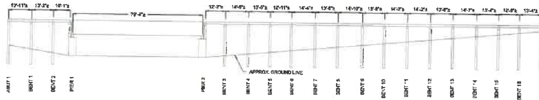
ELEVATION 1 1"=20'-0" S1.0
