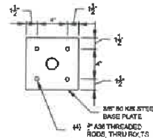
SECTION 1-1 4 1" = 1'-0"
