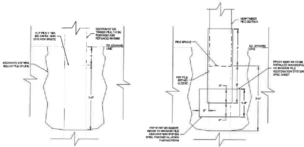
TIMBER PILE SPICE DETAIL 1 1" = 1'-0"
